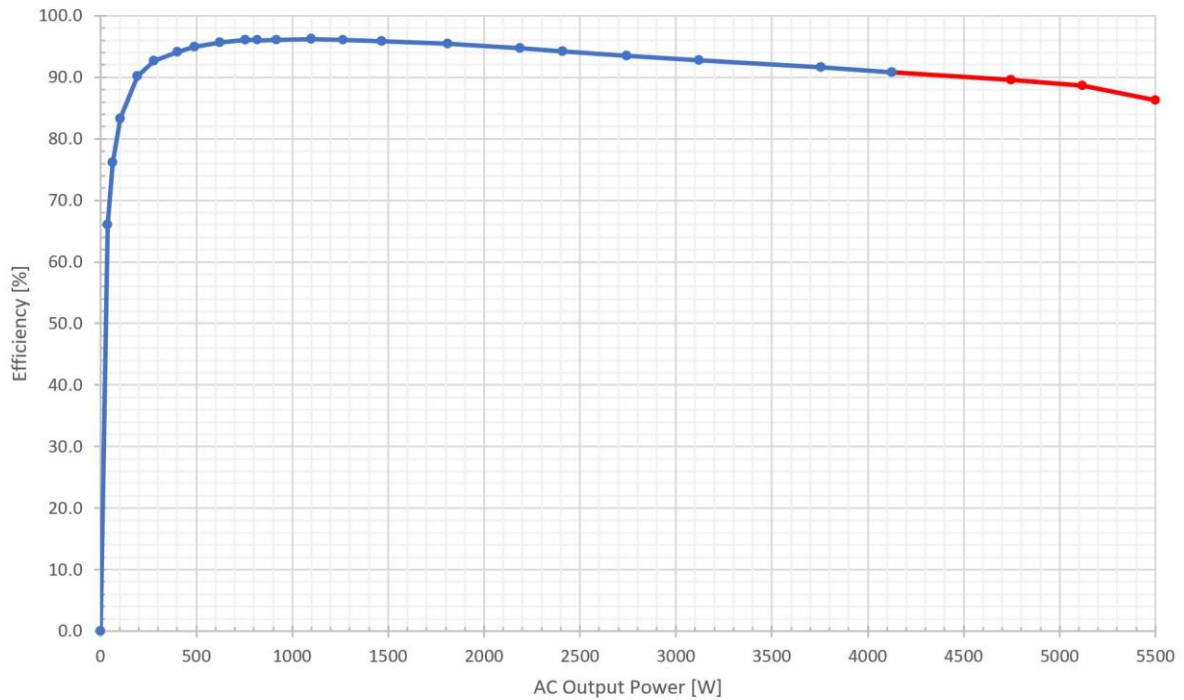
MultiPlus-II 48/5000/70-50
